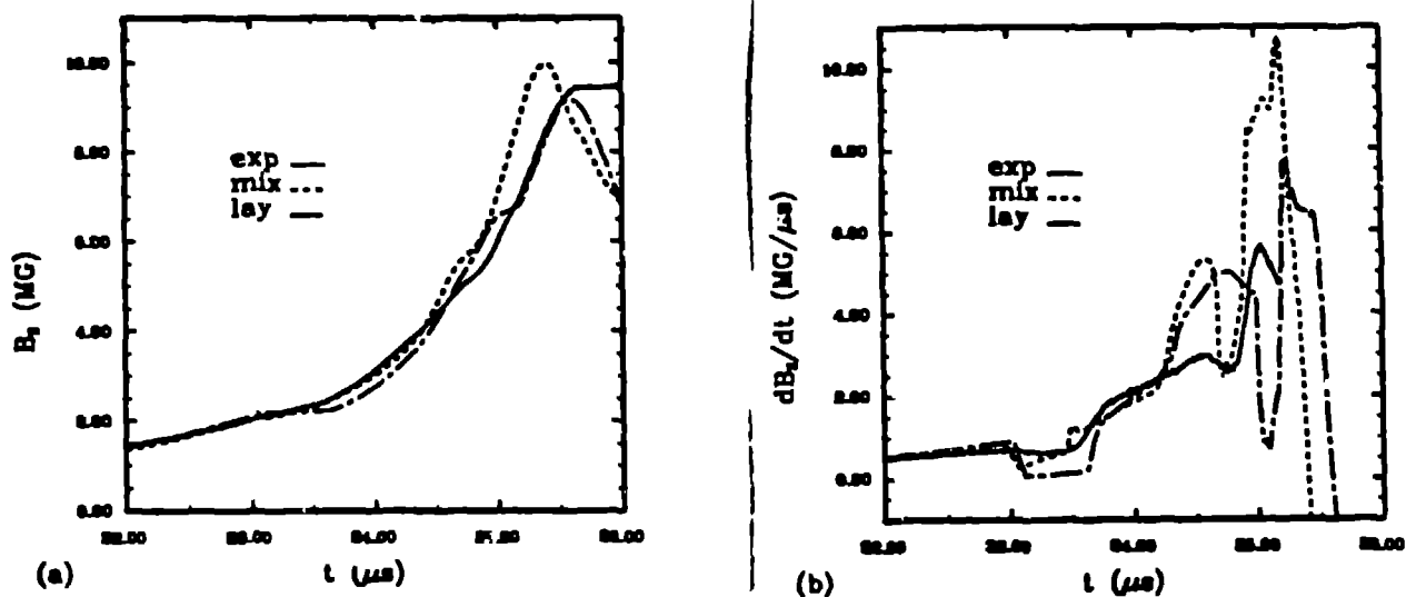
Fig. 4. Calculated field (MG) (a) and field derivative (MG/ \mu\text{s} ) (b) for Comp-B using the mixed EOS and layered model for cascades compared to experimental data.
