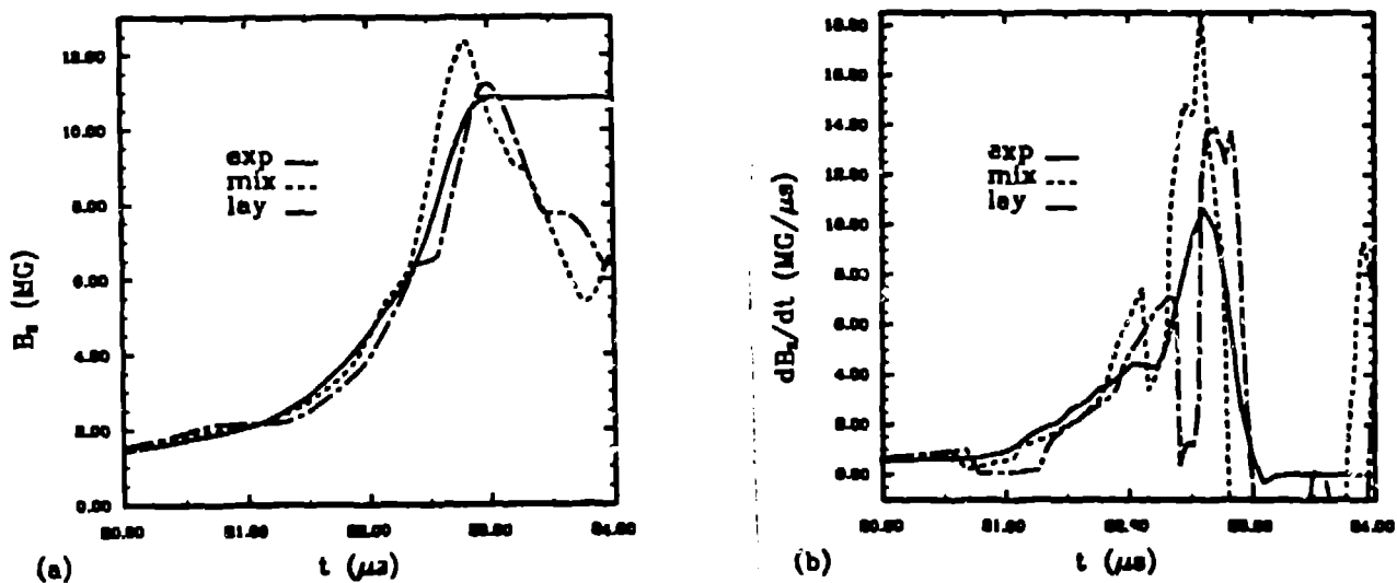
Fig. 5. Calculated field (MG) (a) and field derivative (MG/ \mu\text{s} ) (b) for PBX-9501 using the mixed EOS and layered model for cascades compared to experimental data.
